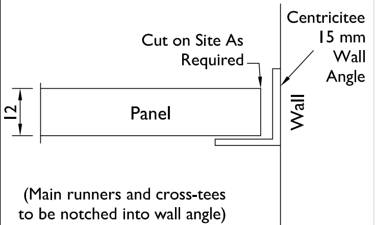
Section Detail 3 + 5 Perimeter Panel to Wall
