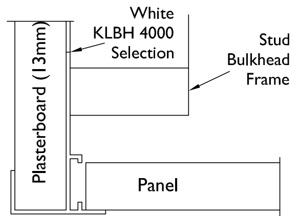
Section Detail 6 Panel to Plasterboard Bulkhead
