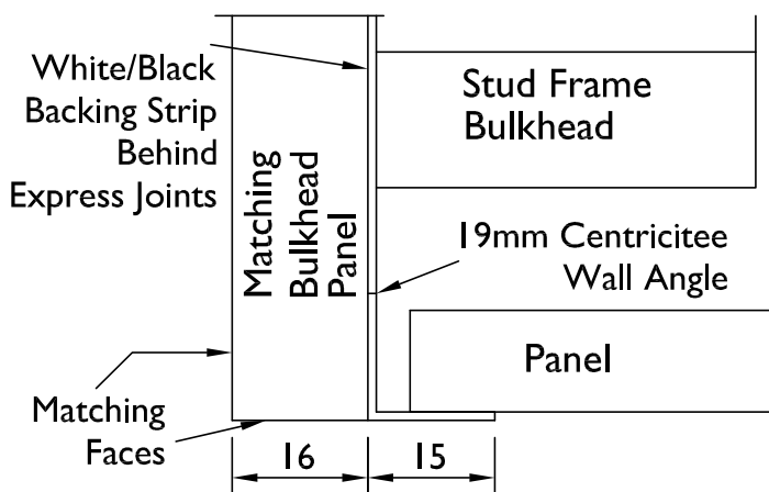
Section Detail 7 Panel to matching Bulkhead
